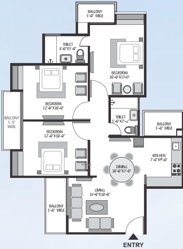
TYPE D - 3BHK/ 2T AREA - 1340 SQ. FT.
